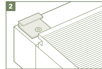
2 STARTER CLIPS: Fitted to the intersection of each joist.
